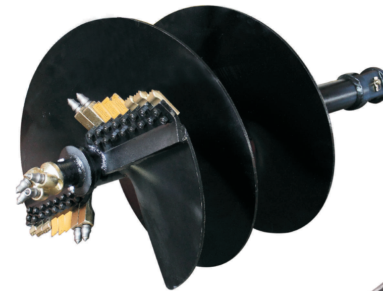
Exchangable Muilt-Founctional Auger
