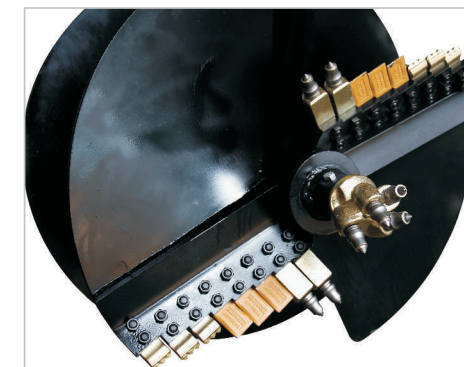
Exchangable Muilt-Founctional Pilot & Bits
